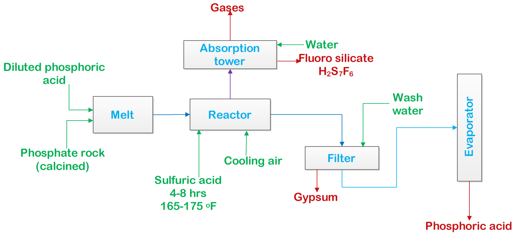
Figure: Manufacturing of Phosphoric acid by Wet process
